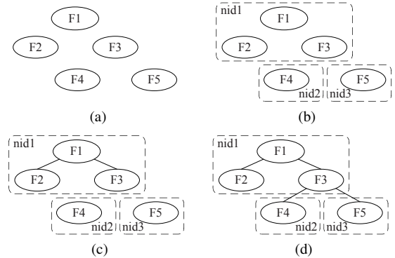
Figure 2. A sample of trace reconstruction in MTracer [1]
